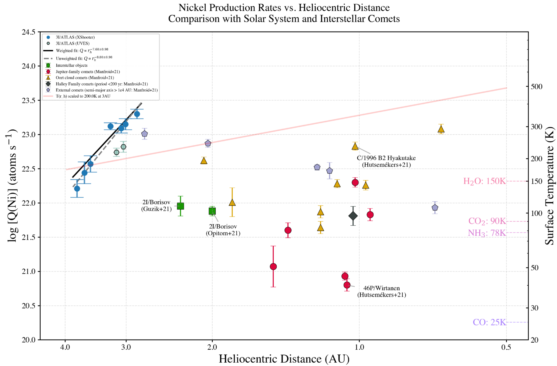
Figure 3. from Rohan Rahatgaonkar et al 2025 Astrophys. J. Lett. 995 doi:10.3847/2041-8213/ae1cbc https://dx.doi.org/10.3847/2041-8213/ae1cbc © 2025. The Author(s). Published by the American Astronomical Society.
