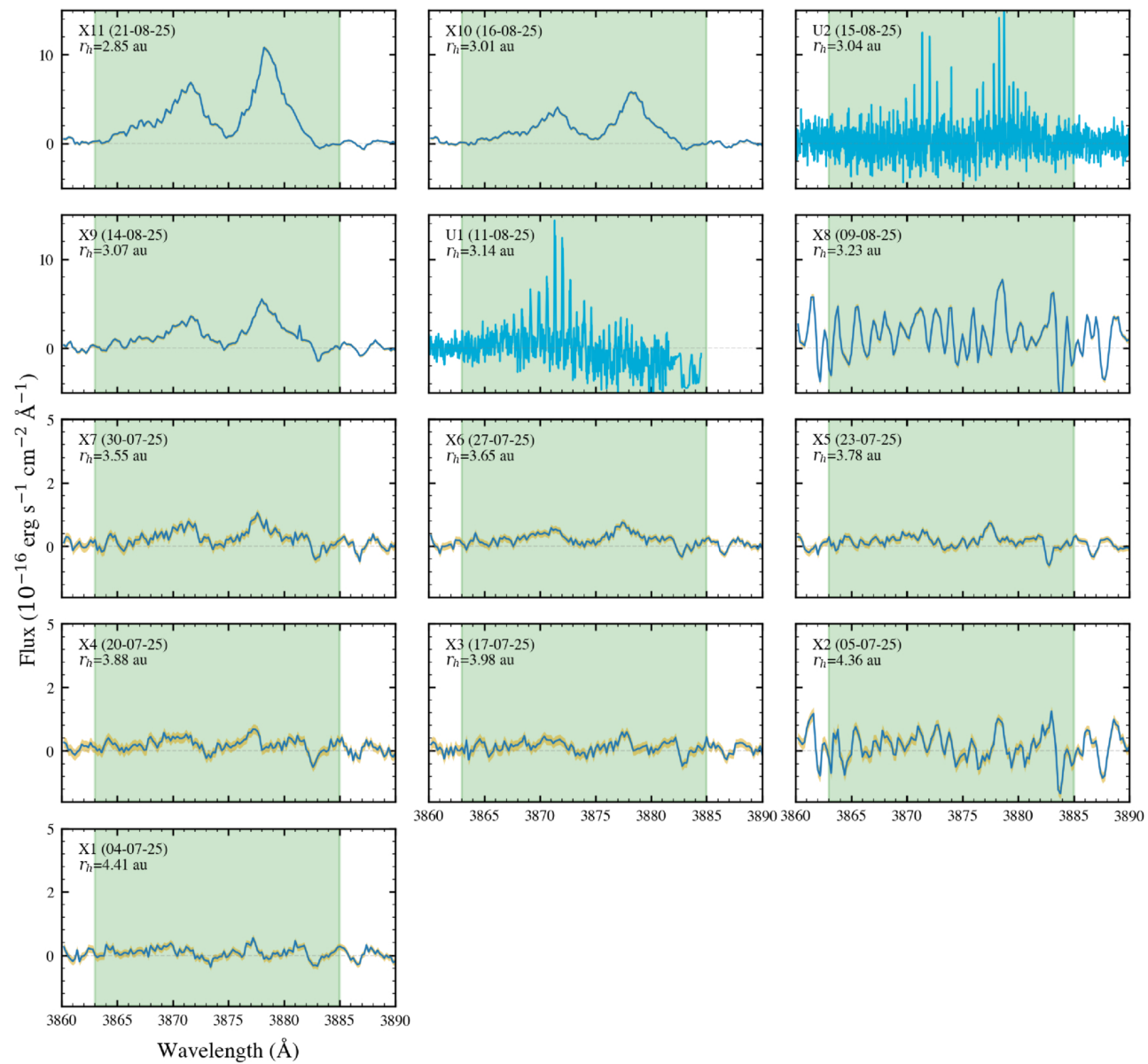
Figure 2. from Rohan Rahatgaonkar et al 2025 Astrophys. J. Lett. 995 doi:10.3847/2041-8213/ae1cbc https://dx.doi.org/10.3847/2041-8213/ae1cbc © 2025. The Author(s). Published by the American Astronomical Society.
