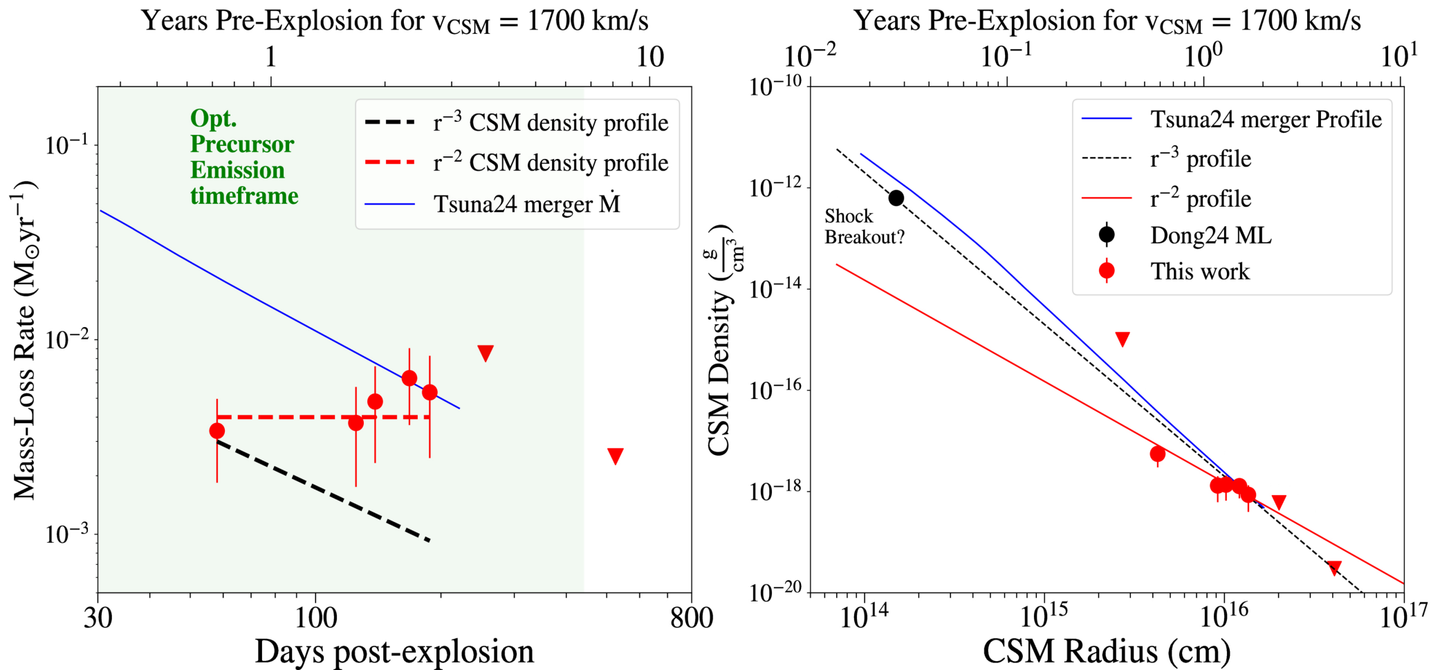
Figure 5. from Raphael Baer-Way et al 2025 Astrophys. J. Lett. 995 doi:10.3847/2041-8213/ae1cb8 https://dx.doi.org/10.3847/2041-8213/ae1cb8 © 2025. The Author(s). Published by the American Astronomical Society.
