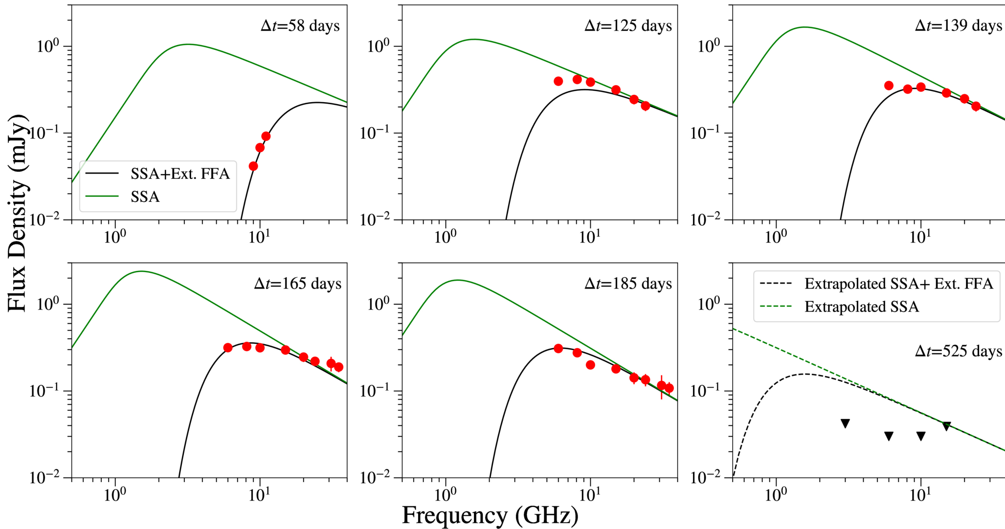
Figure 4. from Raphael Baer-Way et al 2025 Astrophys. J. Lett. 995 doi:10.3847/2041-8213/ae1cb8 https://dx.doi.org/10.3847/2041-8213/ae1cb8 © 2025. The Author(s). Published by the American Astronomical Society.
