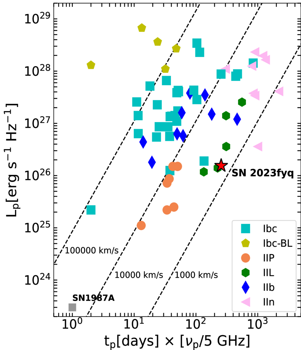
Figure 3. from Raphael Baer-Way et al 2025 Astrophys. J. Lett. 995 doi:10.3847/2041-8213/ae1cb8 https://dx.doi.org/10.3847/2041-8213/ae1cb8 © 2025. The Author(s). Published by the American Astronomical Society.
