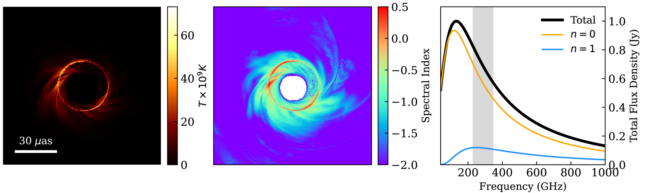
Figure 5. from Daniel C. M. Palumbo et al 2025 Astrophys. J. Lett. 994 doi:10.3847/2041-8213/ae1ba8 https://dx.doi.org/10.3847/2041-8213/ae1ba8 © 2025. The Author(s). Published by the American Astronomical Society.
