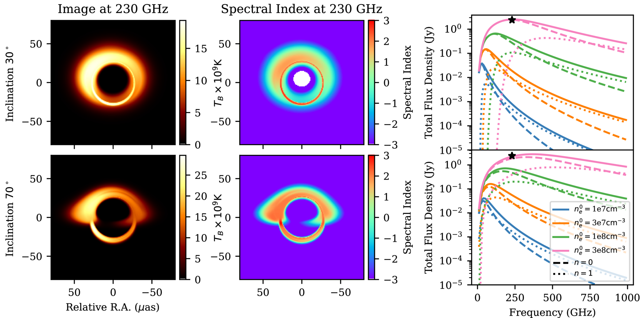
Figure 4. from Daniel C. M. Palumbo et al 2025 Astrophys. J. Lett. 994 doi:10.3847/2041-8213/ae1ba8 https://dx.doi.org/10.3847/2041-8213/ae1ba8 © 2025. The Author(s). Published by the American Astronomical Society.
