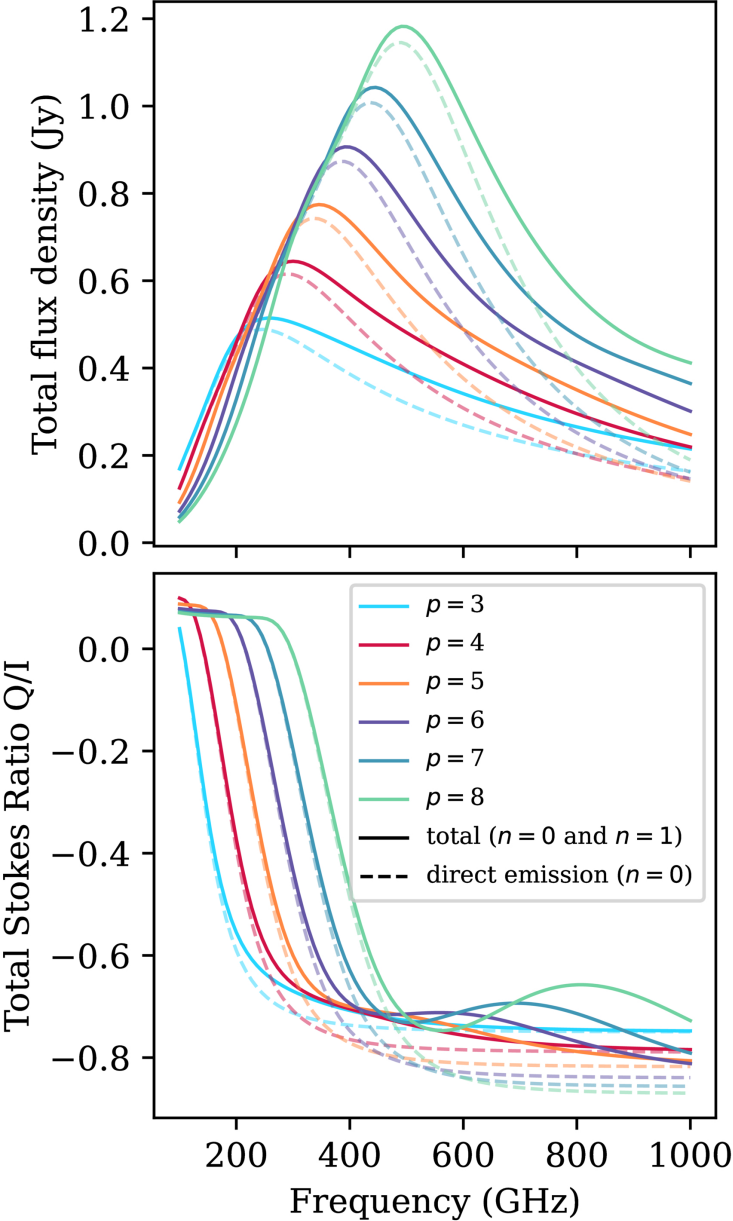
Figure 3. from Daniel C. M. Palumbo et al 2025 Astrophys. J. Lett. 994 doi:10.3847/2041-8213/ae1ba8 https://dx.doi.org/10.3847/2041-8213/ae1ba8 © 2025. The Author(s). Published by the American Astronomical Society.
