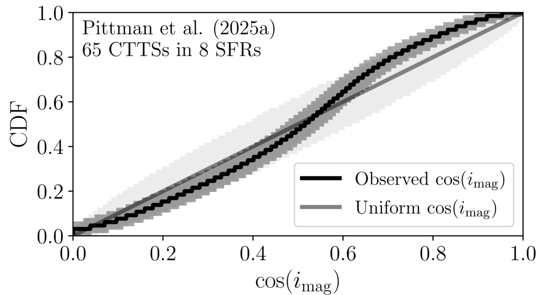
Figure 8. from Caeley V. Pittman et al 2025 Astrophys. J. Lett. 994 doi:10.3847/2041-8213/ae1ba2 https://dx.doi.org/10.3847/2041-8213/ae1ba2 © 2025. The Author(s). Published by the American Astronomical Society.
