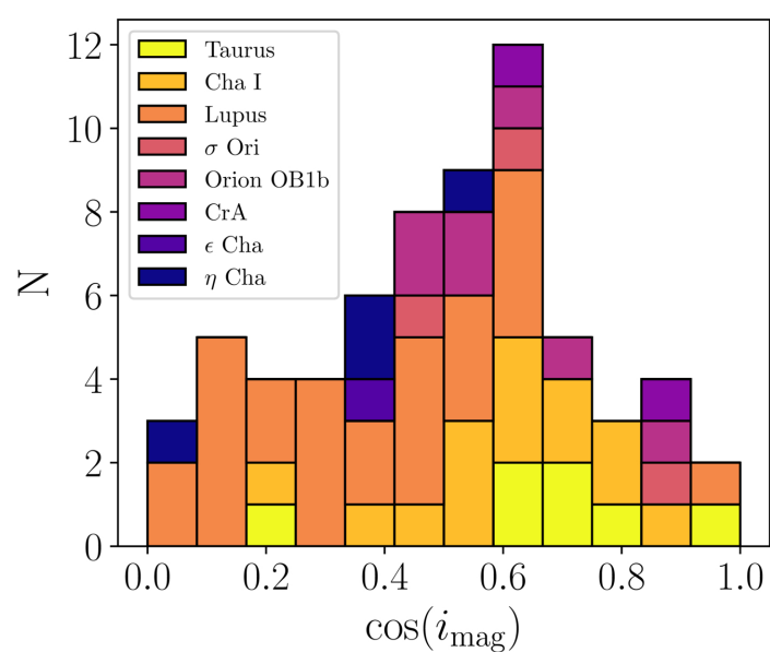
Figure 8. from Caeley V. Pittman et al 2025 Astrophys. J. Lett. 994 doi:10.3847/2041-8213/ae1ba2 https://dx.doi.org/10.3847/2041-8213/ae1ba2 © 2025. The Author(s). Published by the American Astronomical Society.
