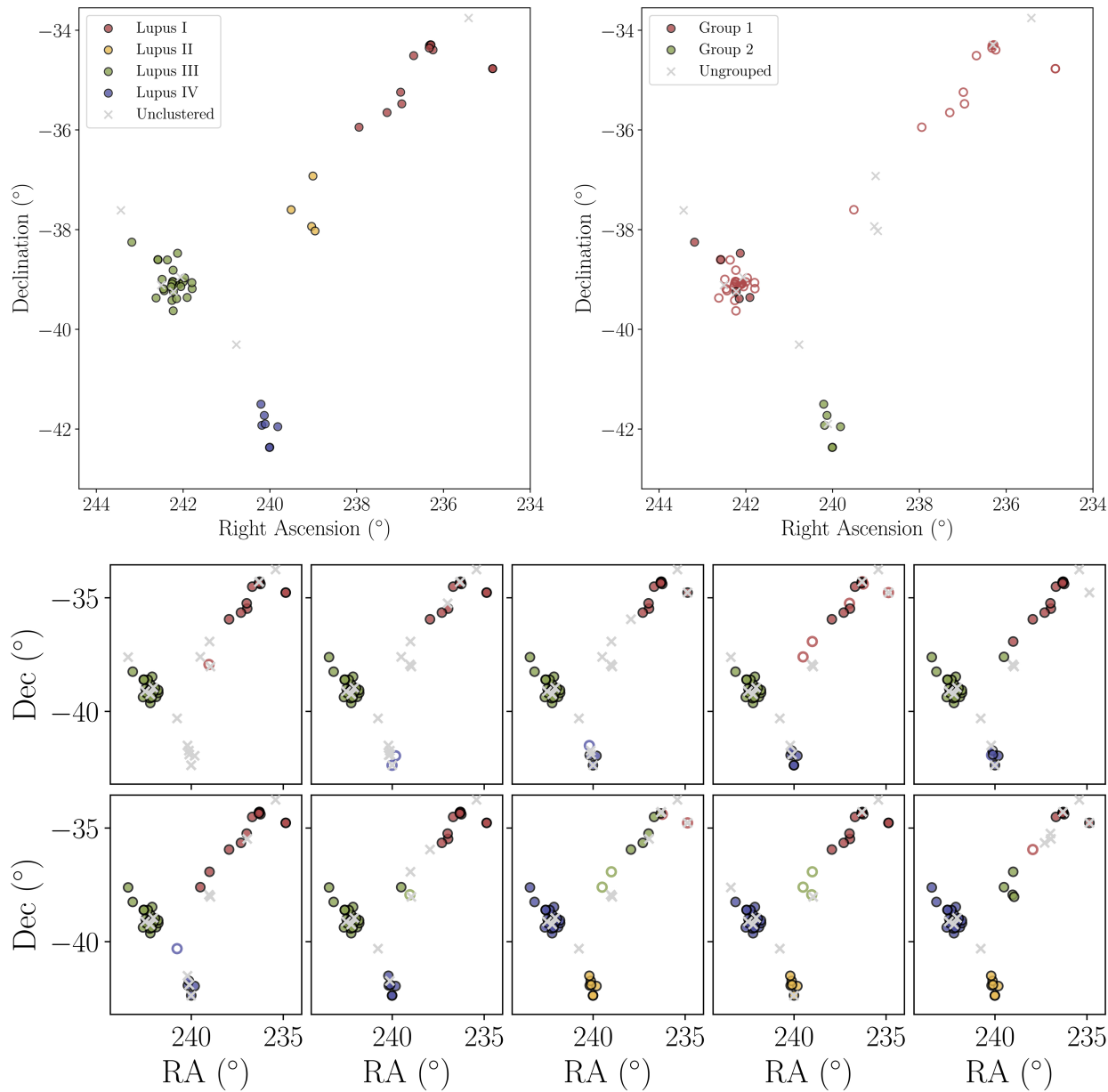
Figure 6. from Caeley V. Pittman et al 2025 Astrophys. J. Lett. 994 doi:10.3847/2041-8213/ae1ba2 https://dx.doi.org/10.3847/2041-8213/ae1ba2 © 2025. The Author(s). Published by the American Astronomical Society.
