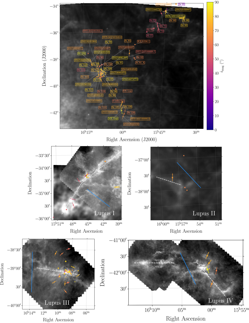
Figure 3. from Caeley V. Pittman et al 2025 Astrophys. J. Lett. 994 doi:10.3847/2041-8213/ae1ba2 https://dx.doi.org/10.3847/2041-8213/ae1ba2 © 2025. The Author(s). Published by the American Astronomical Society.
