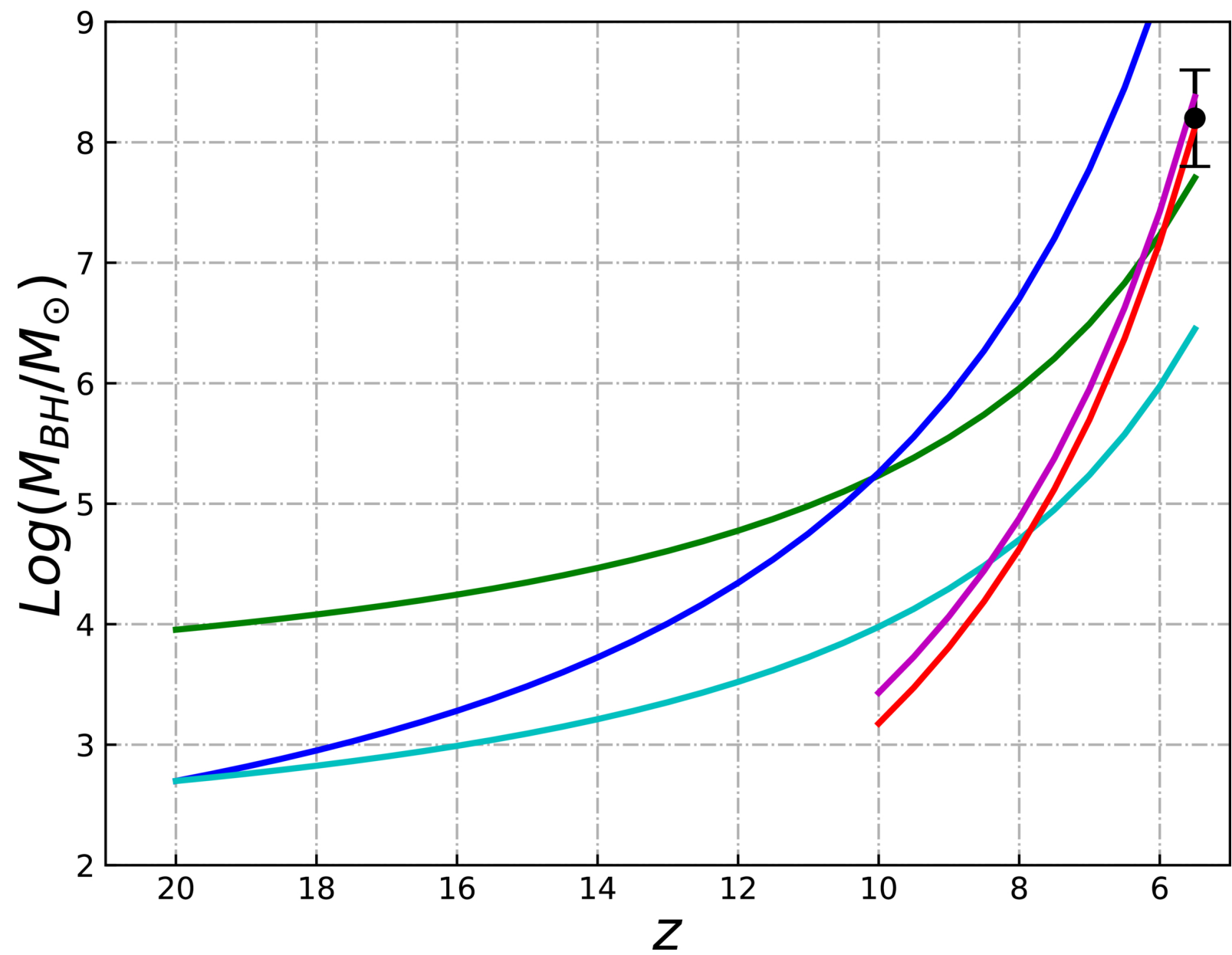
Figure 7. from Devesh Nandal et al 2025 Astrophys. J. Lett. 994 doi:10.3847/2041-8213/ae1a63 https://dx.doi.org/10.3847/2041-8213/ae1a63 © 2025. The Author(s). Published by the American Astronomical Society.
