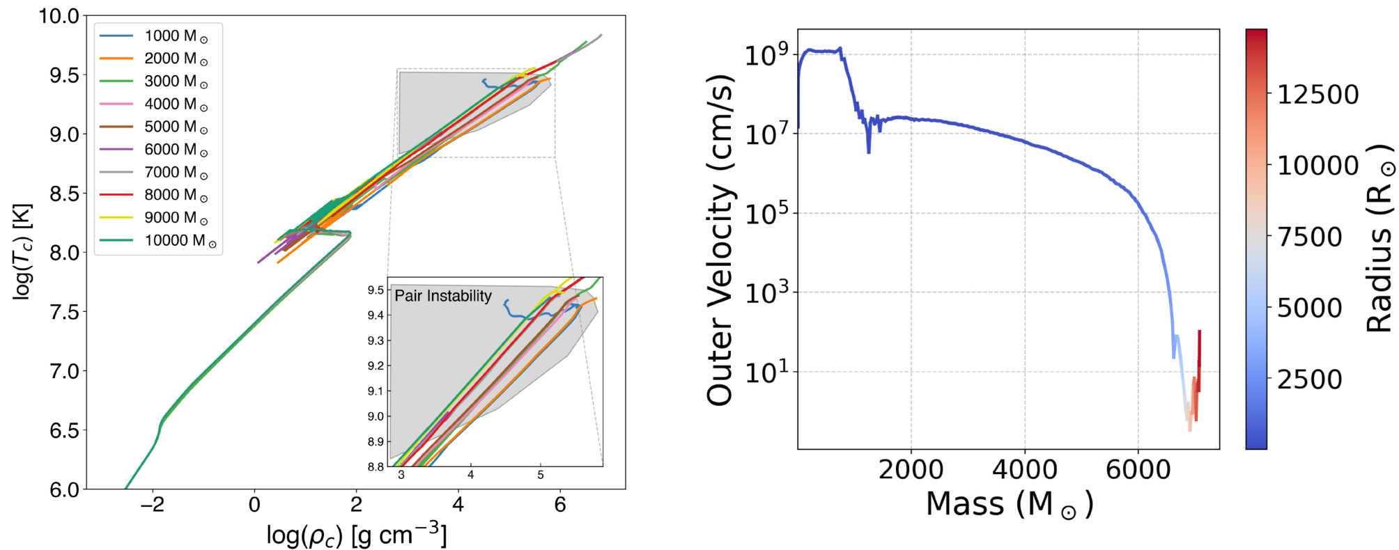
Figure 6. from Devesh Nandal et al 2025 Astrophys. J. Lett. 994 doi:10.3847/2041-8213/ae1a63 https://dx.doi.org/10.3847/2041-8213/ae1a63 © 2025. The Author(s). Published by the American Astronomical Society.
