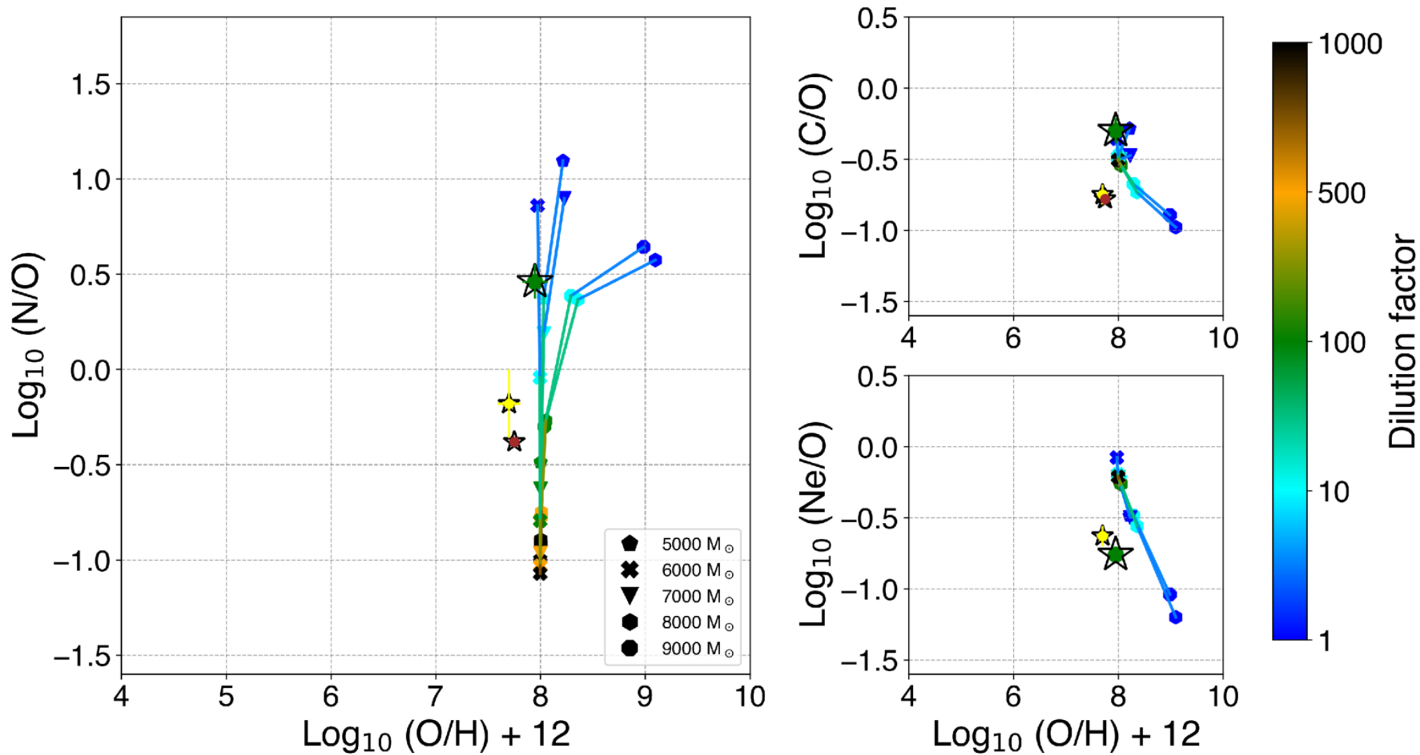
Figure 5. from Devesh Nandal et al 2025 Astrophys. J. Lett. 994 doi:10.3847/2041-8213/ae1a63 https://dx.doi.org/10.3847/2041-8213/ae1a63 © 2025. The Author(s). Published by the American Astronomical Society.
