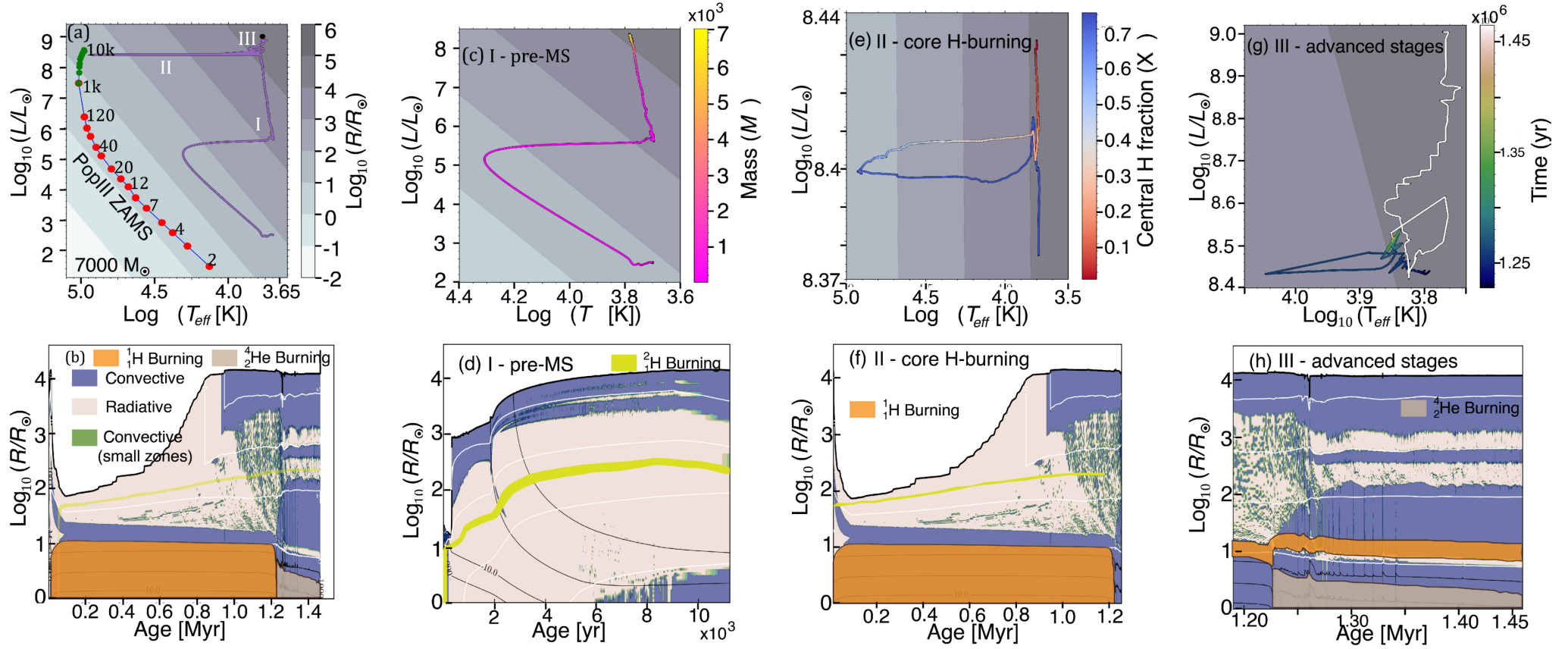
Figure 1. from Devesh Nandal et al 2025 Astrophys. J. Lett. 994 doi:10.3847/2041-8213/ae1a63 https://dx.doi.org/10.3847/2041-8213/ae1a63 © 2025. The Author(s). Published by the American Astronomical Society.
