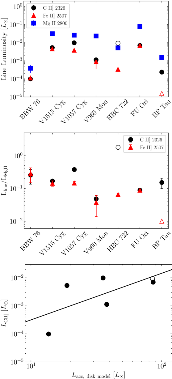
Figure 4. from Adolfo S. Carvalho et al 2025 Astrophys. J. Lett. 994 doi:10.3847/2041-8213/ae1830 https://dx.doi.org/10.3847/2041-8213/ae1830 © 2025. The Author(s). Published by the American Astronomical Society.
