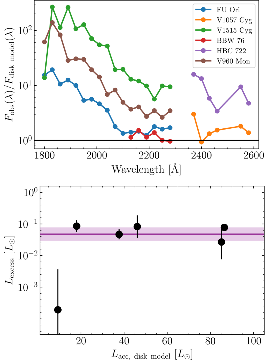
Figure 2. from Adolfo S. Carvalho et al 2025 Astrophys. J. Lett. 994 doi:10.3847/2041-8213/ae1830 https://dx.doi.org/10.3847/2041-8213/ae1830 © 2025. The Author(s). Published by the American Astronomical Society.
