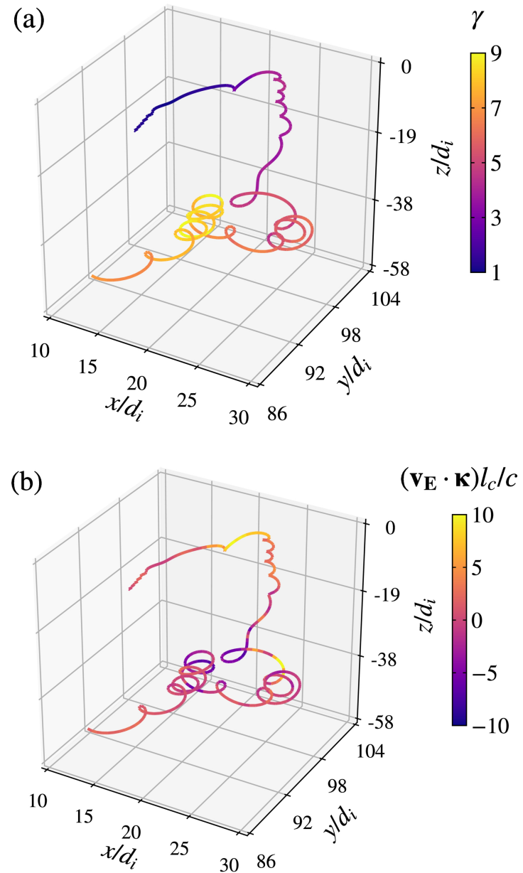
Figure 8. from Samuel T. Sebastian and Luca Comisso 2025 Astrophys. J. Lett. 994 doi:10.3847/2041-8213/ae1696 https://dx.doi.org/10.3847/2041-8213/ae1696 © 2025. The Author(s). Published by the American Astronomical Society.
