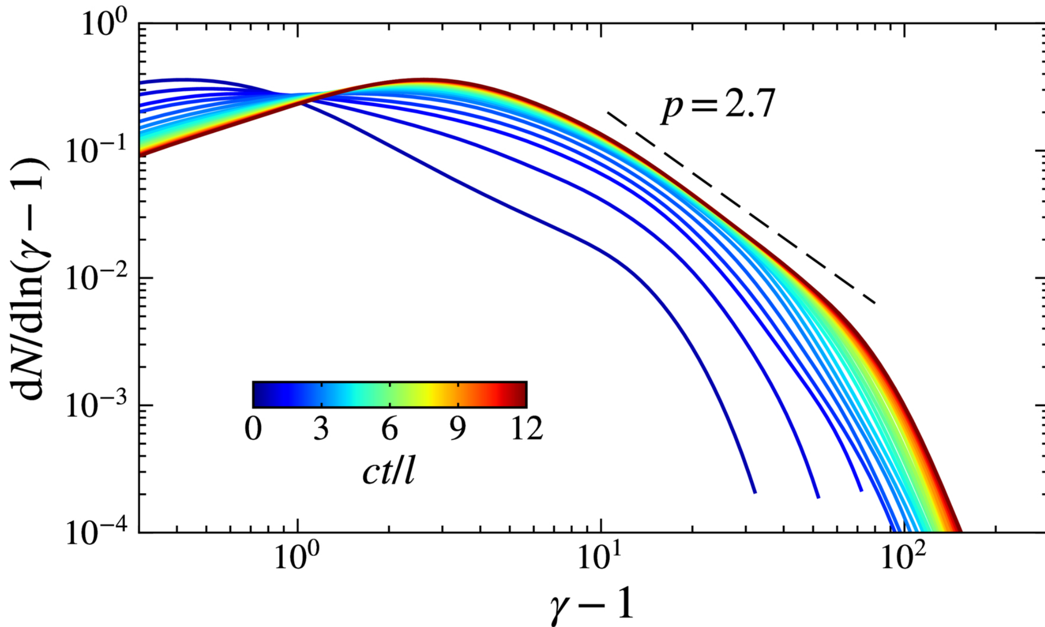
Figure 6. from Samuel T. Sebastian and Luca Comisso 2025 Astrophys. J. Lett. 994 doi:10.3847/2041-8213/ae1696 https://dx.doi.org/10.3847/2041-8213/ae1696 © 2025. The Author(s). Published by the American Astronomical Society.
