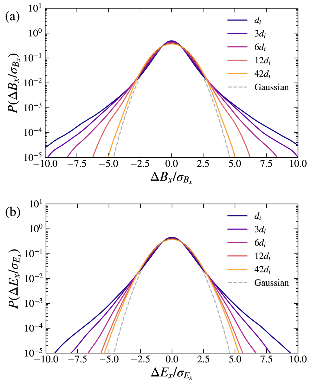
Figure 3. from Samuel T. Sebastian and Luca Comisso 2025 Astrophys. J. Lett. 994 doi:10.3847/2041-8213/ae1696 https://dx.doi.org/10.3847/2041-8213/ae1696 © 2025. The Author(s). Published by the American Astronomical Society.
