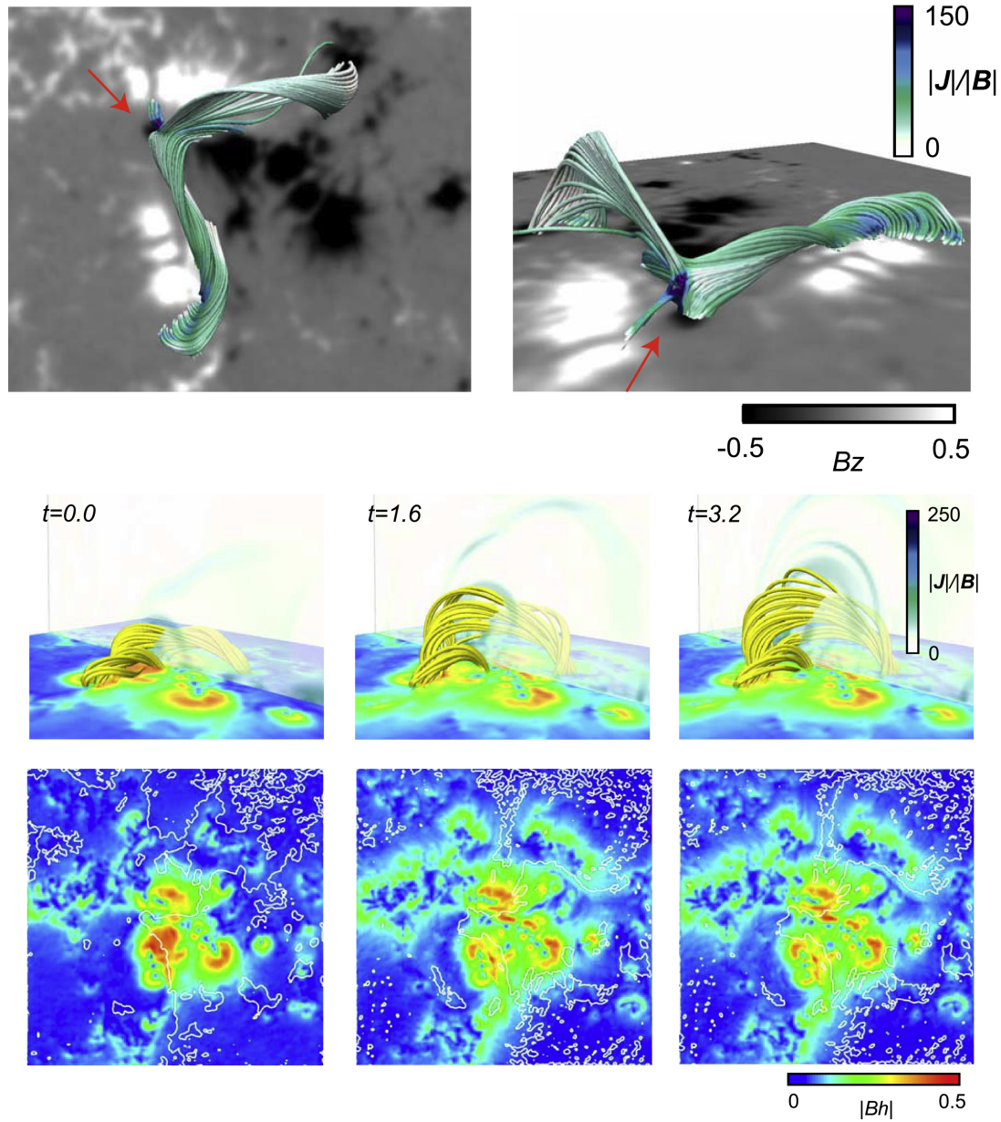
Figure 5. from Ju Jing et al 2025 Astrophys. J. Lett. 993 doi:10.3847/2041-8213/ae160b https://dx.doi.org/10.3847/2041-8213/ae160b © 2025. The Author(s). Published by the American Astronomical Society.
