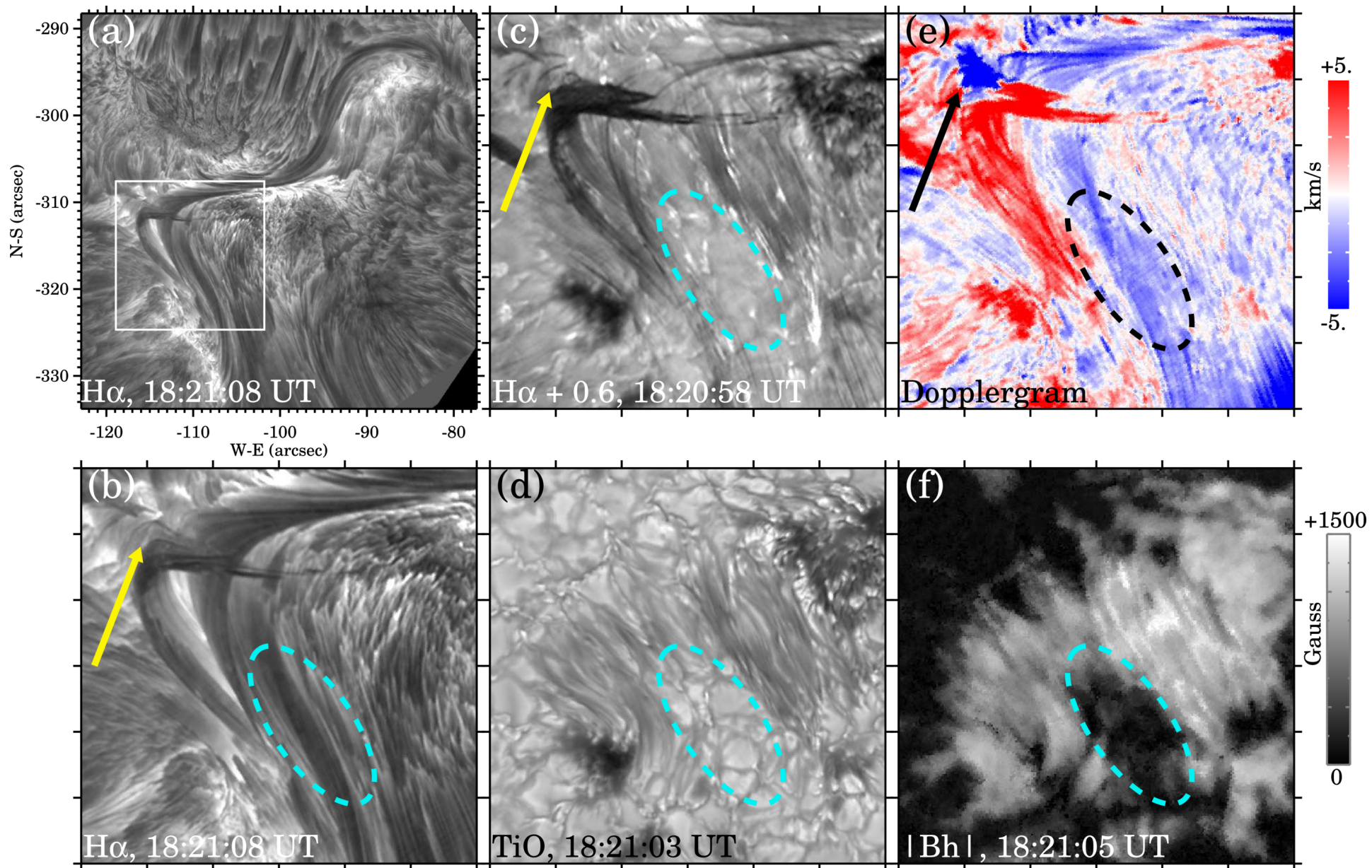
Figure 4. from Ju Jing et al 2025 Astrophys. J. Lett. 993 doi:10.3847/2041-8213/ae160b https://dx.doi.org/10.3847/2041-8213/ae160b © 2025. The Author(s). Published by the American Astronomical Society.
