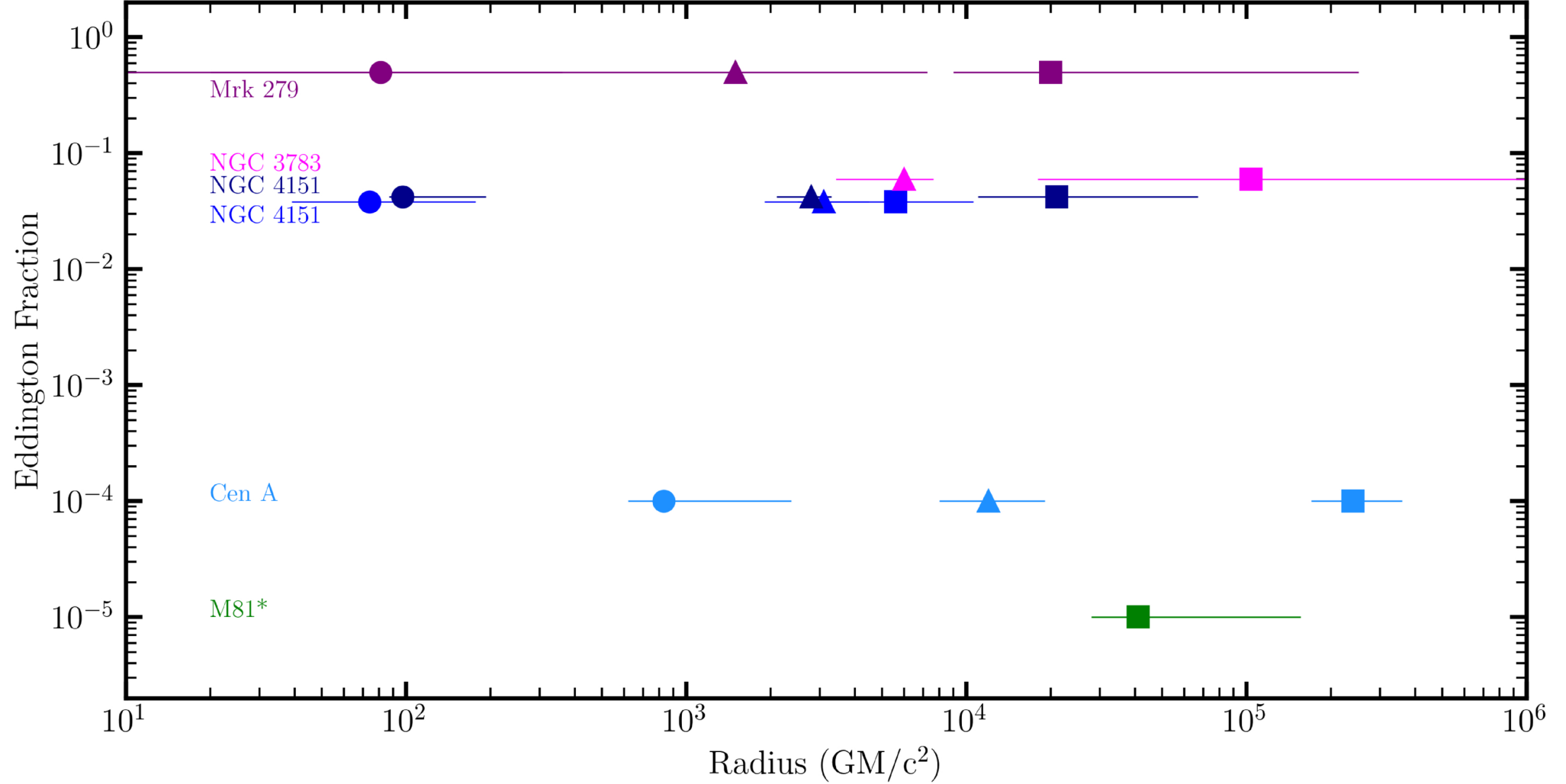
Figure 5. from Jon M. Miller et al 2025 Astrophys. J. Lett. 994 doi:10.3847/2041-8213/ae1606 https://dx.doi.org/10.3847/2041-8213/ae1606 © 2025. The Author(s). Published by the American Astronomical Society.
