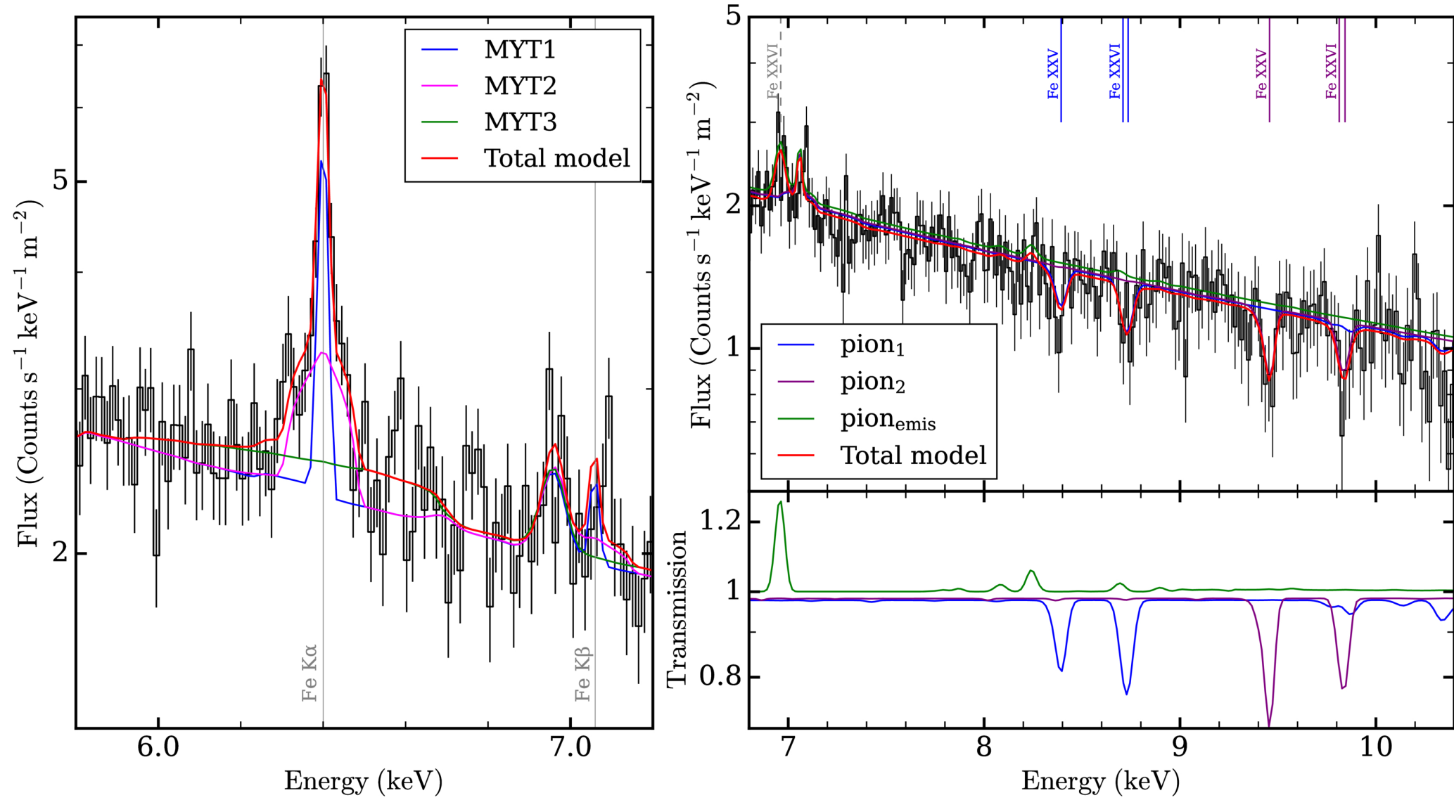
Figure 4. from Jon M. Miller et al 2025 Astrophys. J. Lett. 994 doi:10.3847/2041-8213/ae1606 https://dx.doi.org/10.3847/2041-8213/ae1606 © 2025. The Author(s). Published by the American Astronomical Society.
