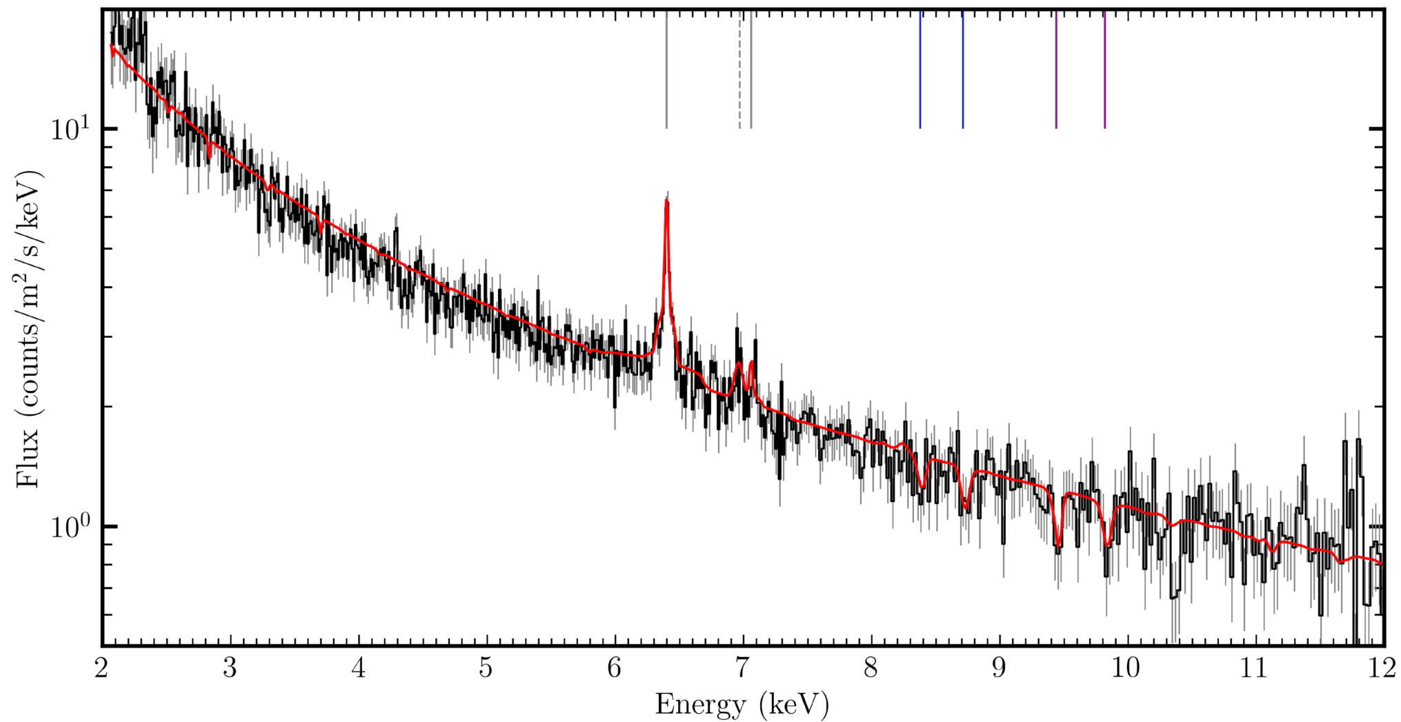
Figure 3. from Jon M. Miller et al 2025 Astrophys. J. Lett. 994 doi:10.3847/2041-8213/ae1606 https://dx.doi.org/10.3847/2041-8213/ae1606 © 2025. The Author(s). Published by the American Astronomical Society.
