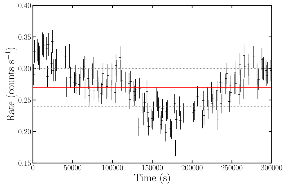
Figure 1. from Jon M. Miller et al 2025 Astrophys. J. Lett. 994 doi:10.3847/2041-8213/ae1606 https://dx.doi.org/10.3847/2041-8213/ae1606 © 2025. The Author(s). Published by the American Astronomical Society.
