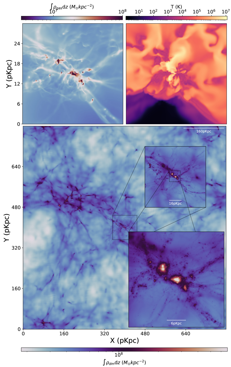
Figure 1. from Ziyong Wu et al 2025 Astrophys. J. Lett. 993 doi:10.3847/2041-8213/ae14d4 https://dx.doi.org/10.3847/2041-8213/ae14d4 © 2025. The Author(s). Published by the American Astronomical Society.
