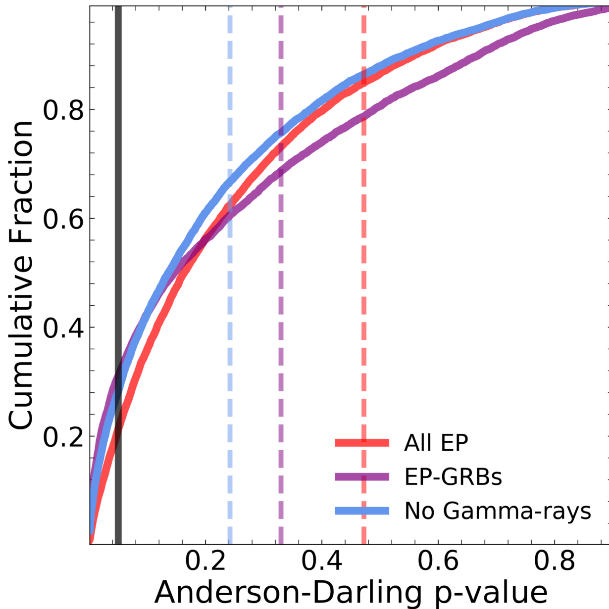
Figure C2. from Brendan O'Connor et al 2025 Astrophys. J. Lett. 993 doi:10.3847/2041-8213/ae146b https://dx.doi.org/10.3847/2041-8213/ae146b © 2025. The Author(s). Published by the American Astronomical Society.
