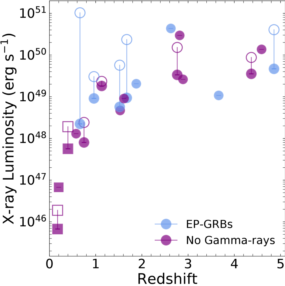
Figure 3. from Brendan O'Connor et al 2025 Astrophys. J. Lett. 993 doi:10.3847/2041-8213/ae146b https://dx.doi.org/10.3847/2041-8213/ae146b © 2025. The Author(s). Published by the American Astronomical Society.
