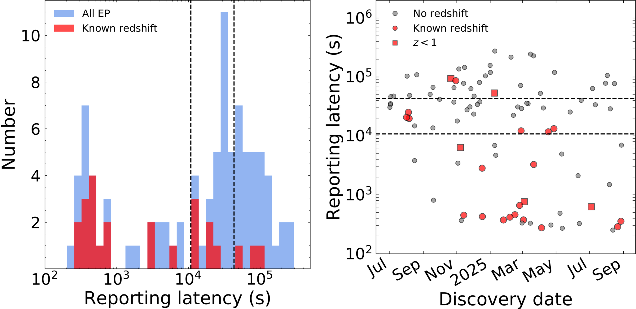
Figure 1. from Brendan O'Connor et al 2025 Astrophys. J. Lett. 993 doi:10.3847/2041-8213/ae146b https://dx.doi.org/10.3847/2041-8213/ae146b © 2025. The Author(s). Published by the American Astronomical Society.
