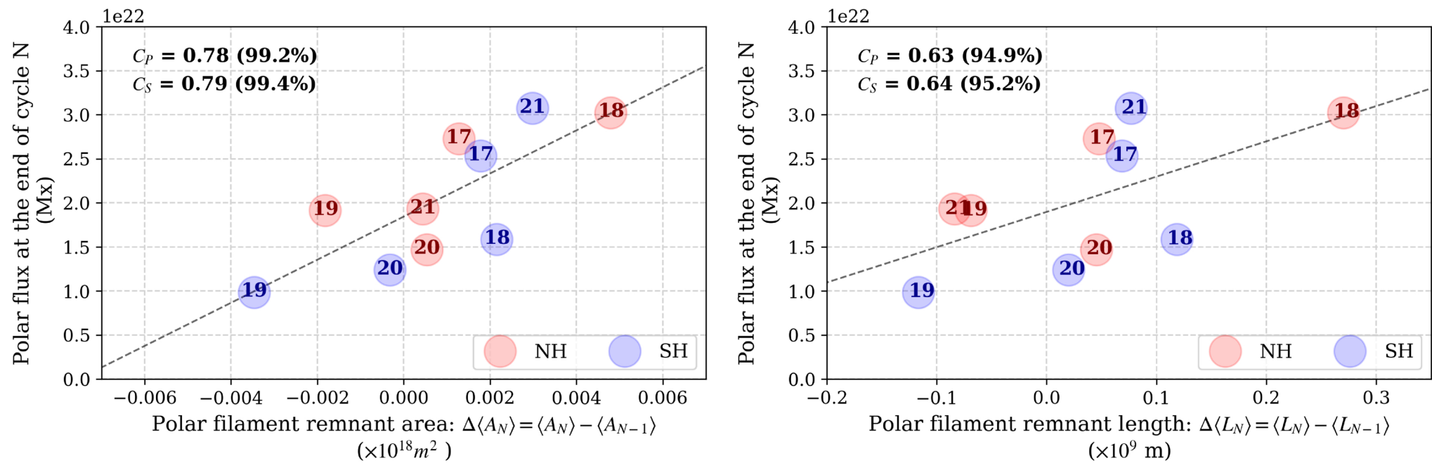
Figure 4. from Srinjana Routh et al 2025 Astrophys. J. Lett. 993 doi:10.3847/2041-8213/ae146a https://dx.doi.org/10.3847/2041-8213/ae146a © 2025. The Author(s). Published by the American Astronomical Society.
