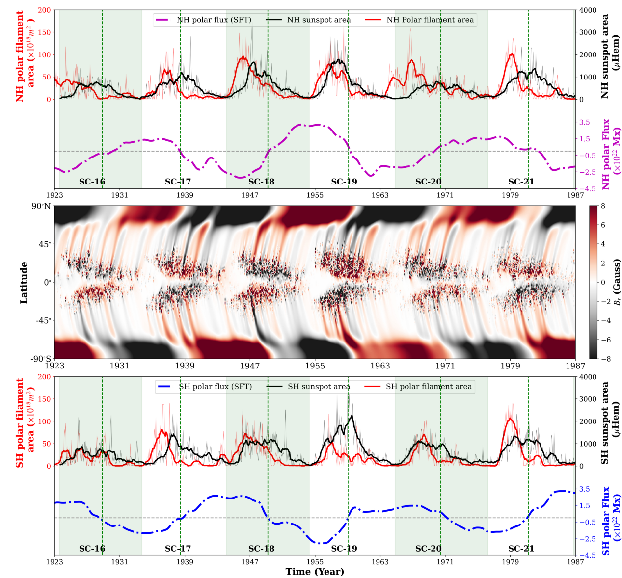
Figure 3. from Srinjana Routh et al 2025 Astrophys. J. Lett. 993 doi:10.3847/2041-8213/ae146a https://dx.doi.org/10.3847/2041-8213/ae146a © 2025. The Author(s). Published by the American Astronomical Society.
