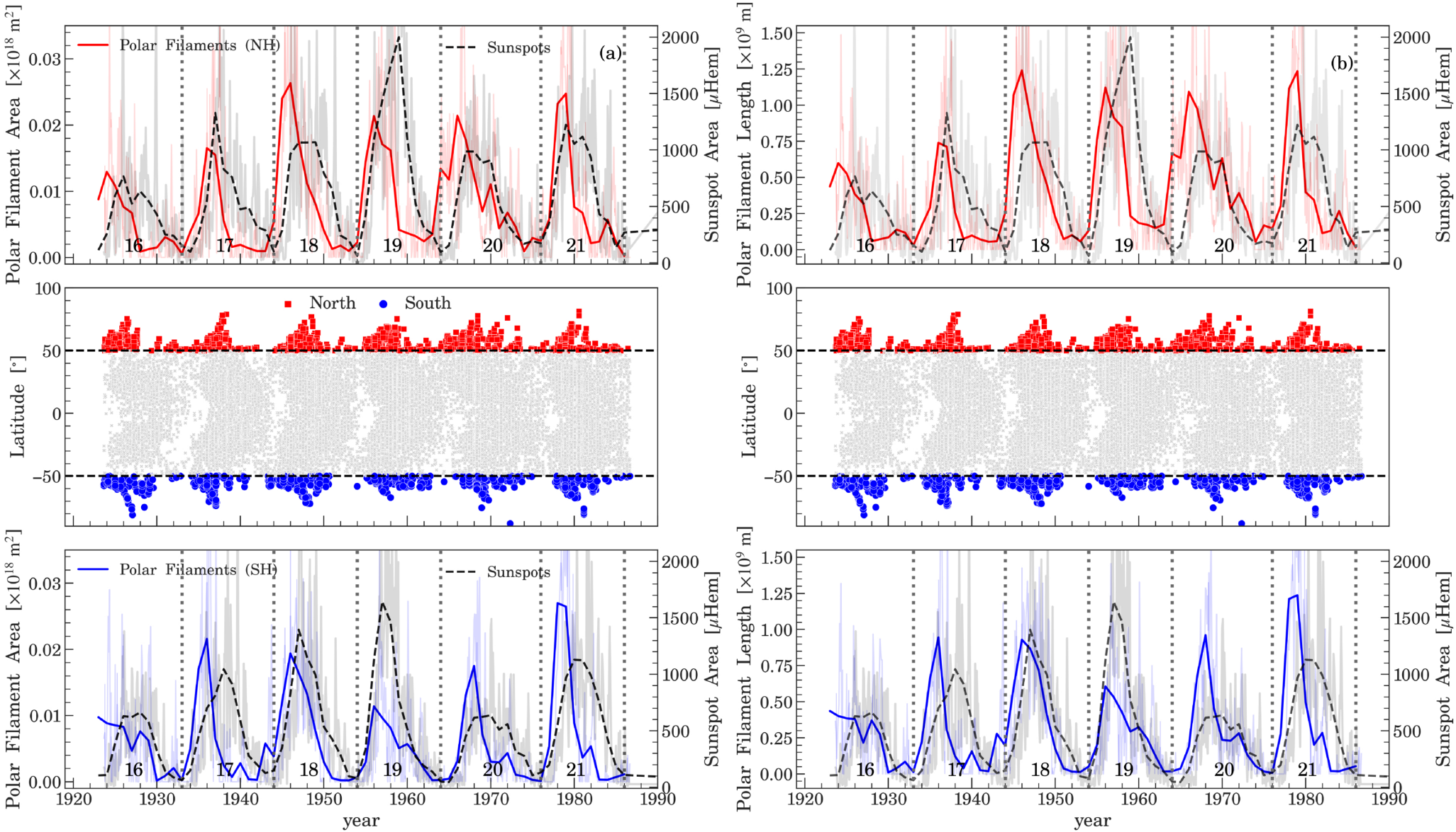
Figure 2. from Srinjana Routh et al 2025 Astrophys. J. Lett. 993 doi:10.3847/2041-8213/ae146a https://dx.doi.org/10.3847/2041-8213/ae146a © 2025. The Author(s). Published by the American Astronomical Society.
