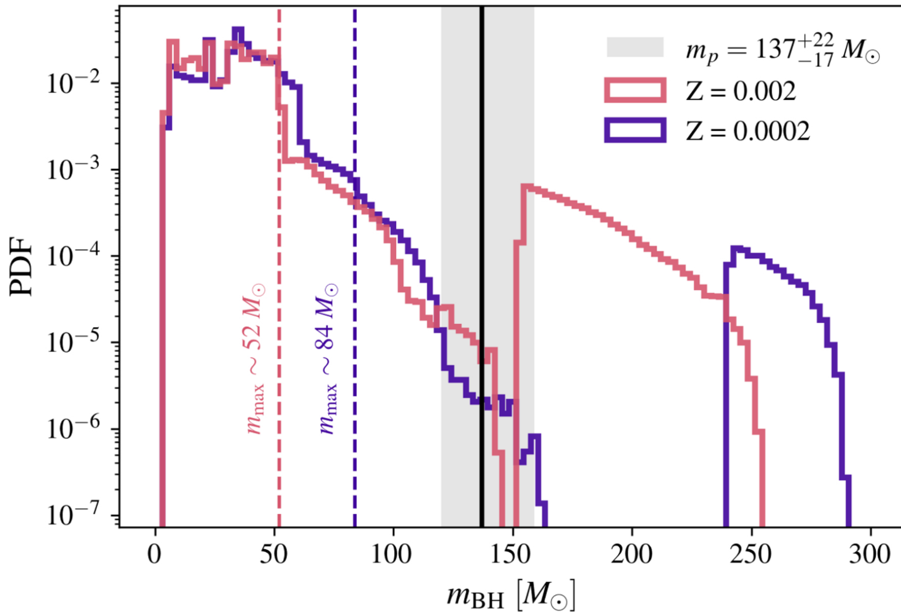
Figure 6. from Lavinia Paiella et al 2025 Astrophys. J. Lett. 994 doi:10.3847/2041-8213/ae1447 https://dx.doi.org/10.3847/2041-8213/ae1447 © 2025. The Author(s). Published by the American Astronomical Society.
