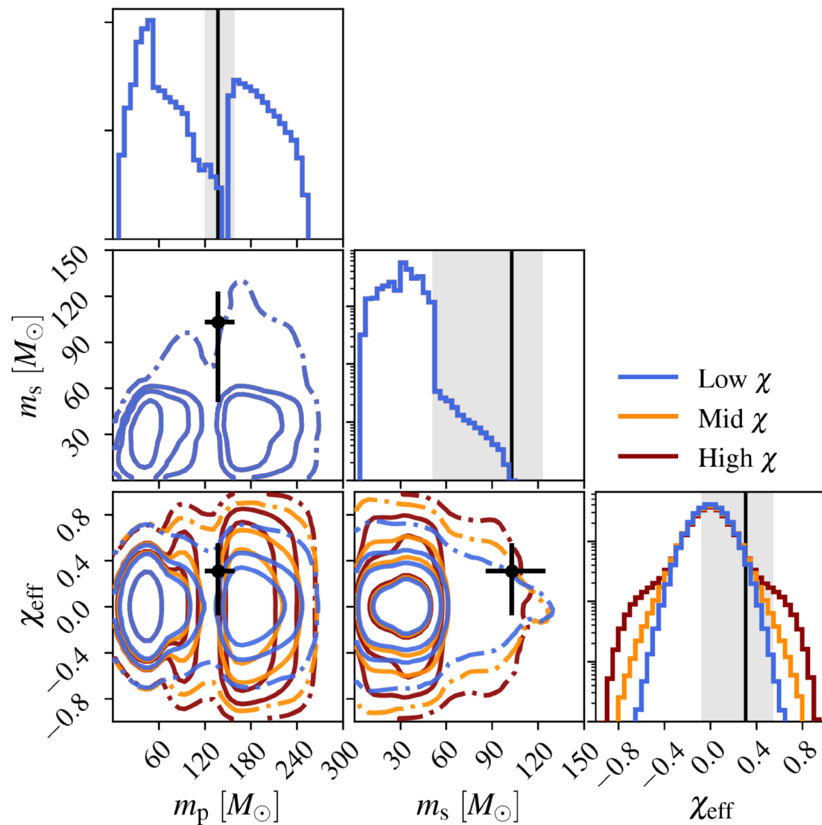
Figure 4. from Lavinia Paiella et al 2025 Astrophys. J. Lett. 994 doi:10.3847/2041-8213/ae1447 https://dx.doi.org/10.3847/2041-8213/ae1447 © 2025. The Author(s). Published by the American Astronomical Society.
