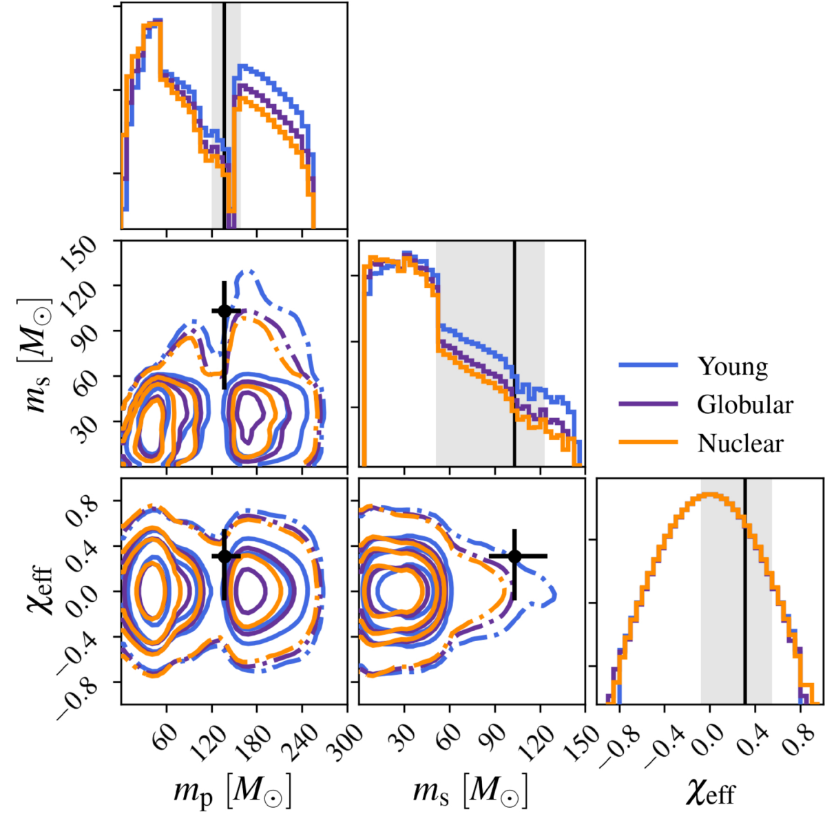
Figure 3. from Lavinia Paiella et al 2025 Astrophys. J. Lett. 994 doi:10.3847/2041-8213/ae1447 https://dx.doi.org/10.3847/2041-8213/ae1447 © 2025. The Author(s). Published by the American Astronomical Society.
