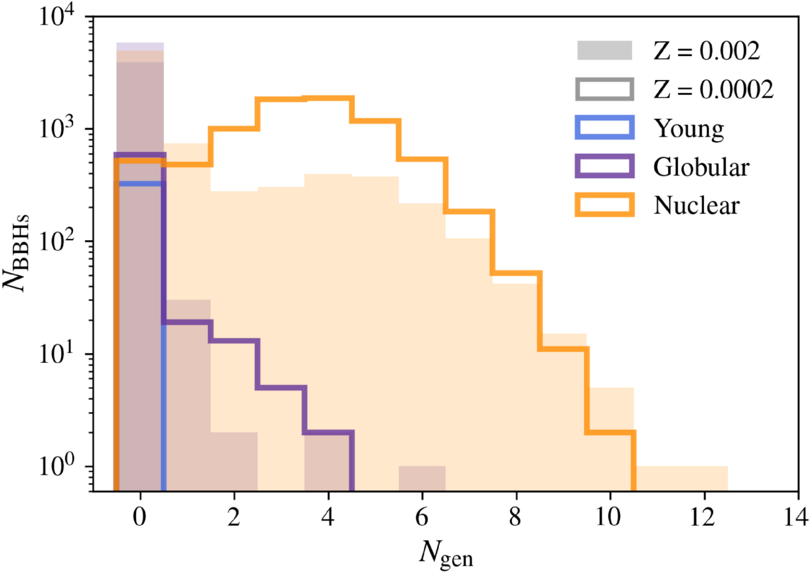
Figure 2. from Lavinia Paiella et al 2025 Astrophys. J. Lett. 994 doi:10.3847/2041-8213/ae1447 https://dx.doi.org/10.3847/2041-8213/ae1447 © 2025. The Author(s). Published by the American Astronomical Society.
