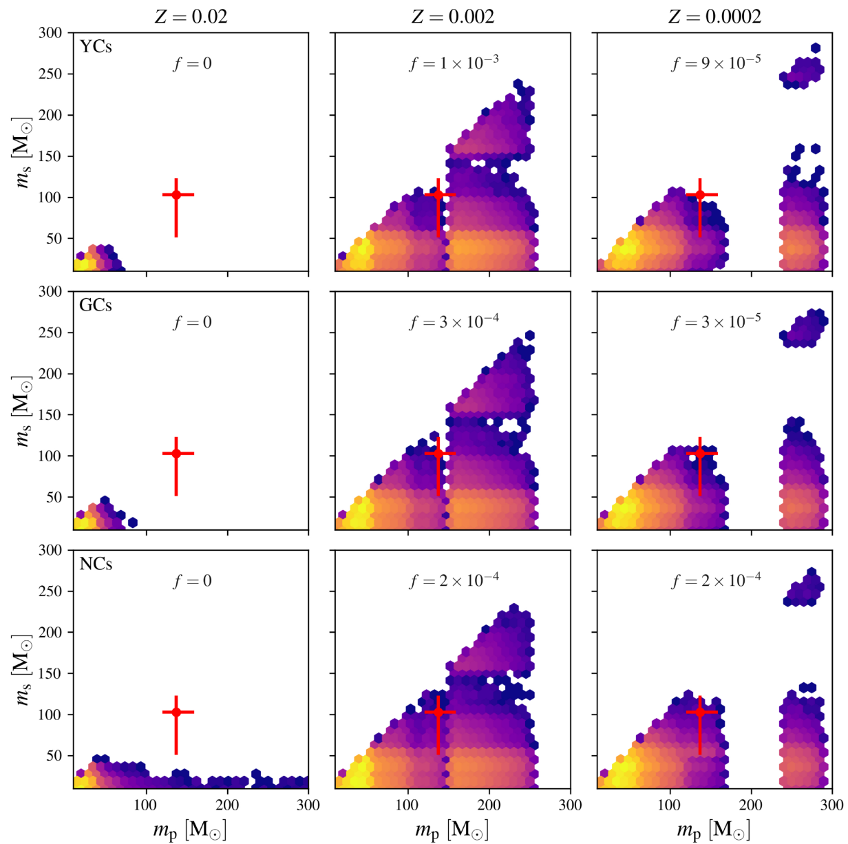
Figure 1. from Lavinia Paiella et al 2025 Astrophys. J. Lett. 994 doi:10.3847/2041-8213/ae1447 https://dx.doi.org/10.3847/2041-8213/ae1447 © 2025. The Author(s). Published by the American Astronomical Society.
