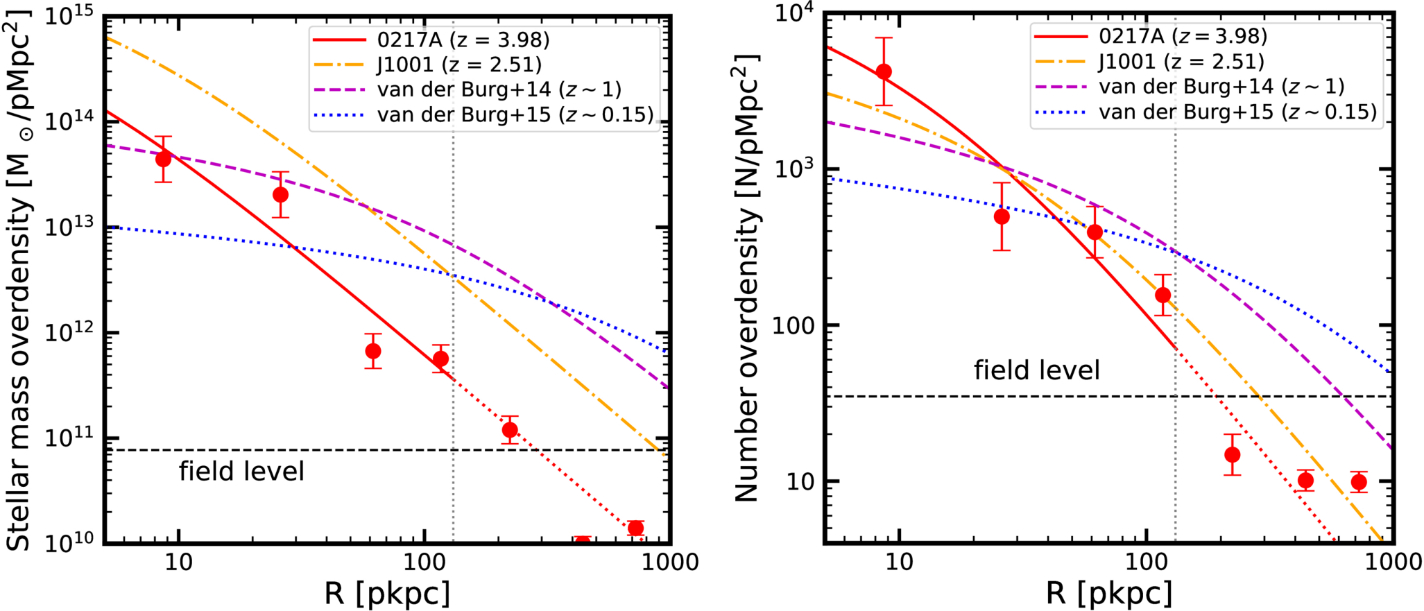
Figure 5. from Hanwen Sun et al 2025 Astrophys. J. Lett. 993 doi:10.3847/2041-8213/ae1132 https://dx.doi.org/10.3847/2041-8213/ae1132 © 2025. The Author(s). Published by the American Astronomical Society.
