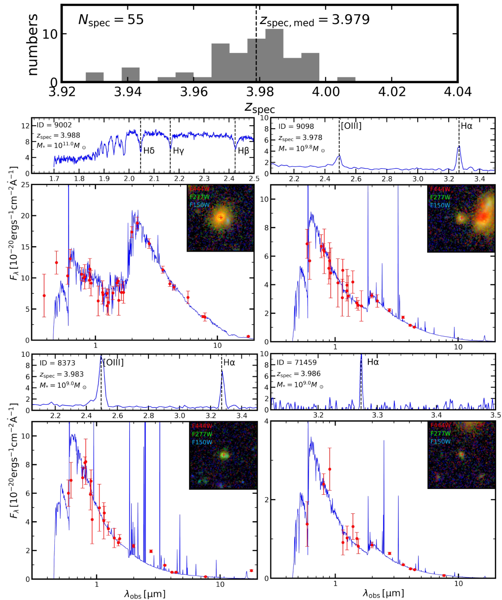
Figure 2. from Hanwen Sun et al 2025 Astrophys. J. Lett. 993 doi:10.3847/2041-8213/ae1132 https://dx.doi.org/10.3847/2041-8213/ae1132 © 2025. The Author(s). Published by the American Astronomical Society.
