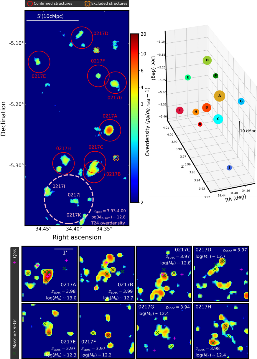
Figure 1. from Hanwen Sun et al 2025 Astrophys. J. Lett. 993 doi:10.3847/2041-8213/ae1132 https://dx.doi.org/10.3847/2041-8213/ae1132 © 2025. The Author(s). Published by the American Astronomical Society.
