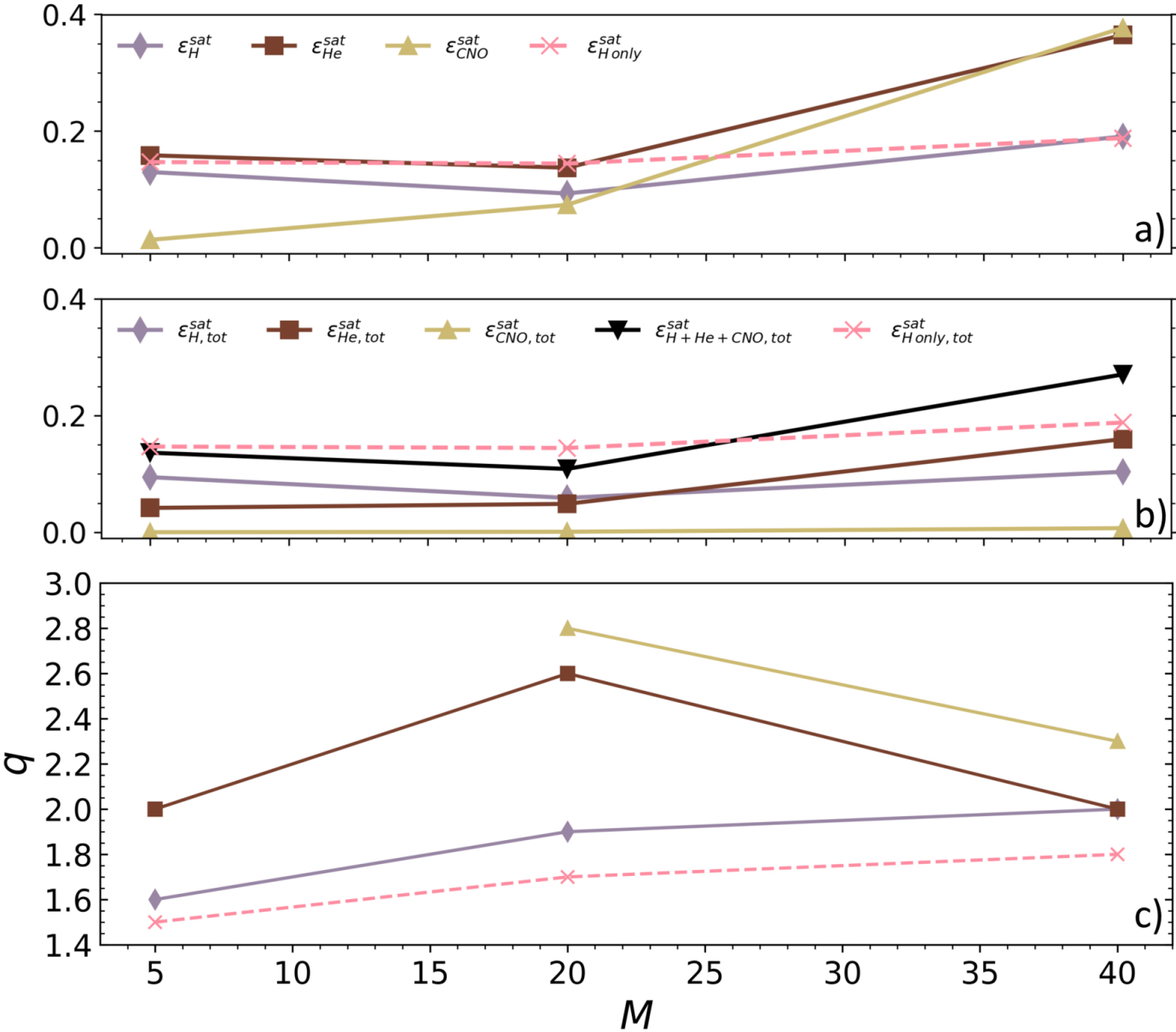
Figure 3. from Damiano Caprioli et al 2025 Astrophys. J. Lett. 993 doi:10.3847/2041-8213/ae109b https://dx.doi.org/10.3847/2041-8213/ae109b © 2025. The Author(s). Published by the American Astronomical Society.
