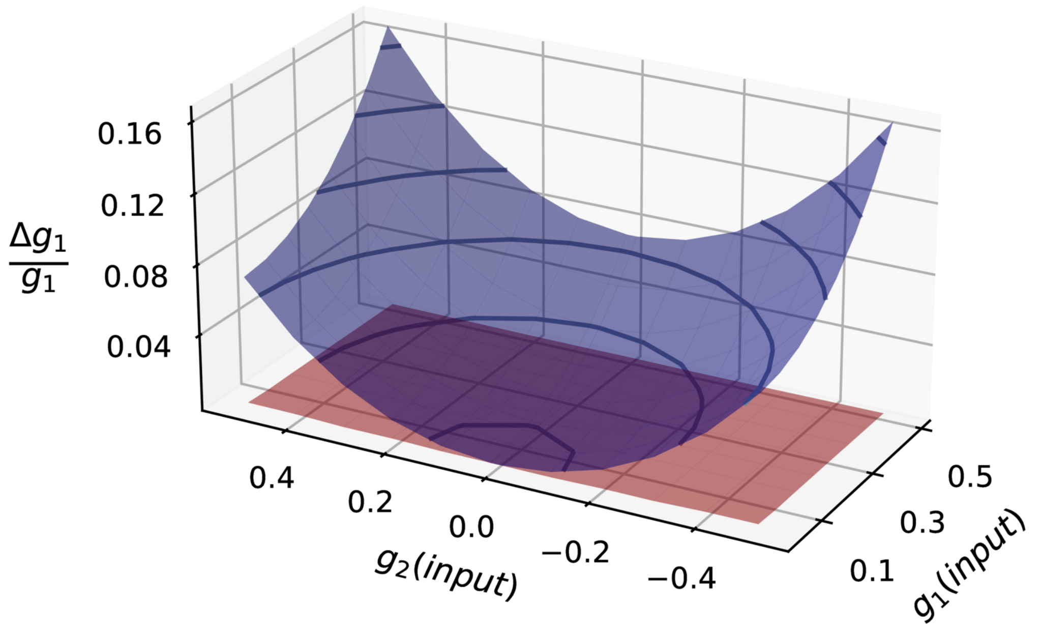
Figure 1. from Jiarui Sun et al 2025 Astrophys. J. Lett. 992 doi:10.3847/2041-8213/ae0f16 https://dx.doi.org/10.3847/2041-8213/ae0f16 © 2025. The Author(s). Published by the American Astronomical Society.
