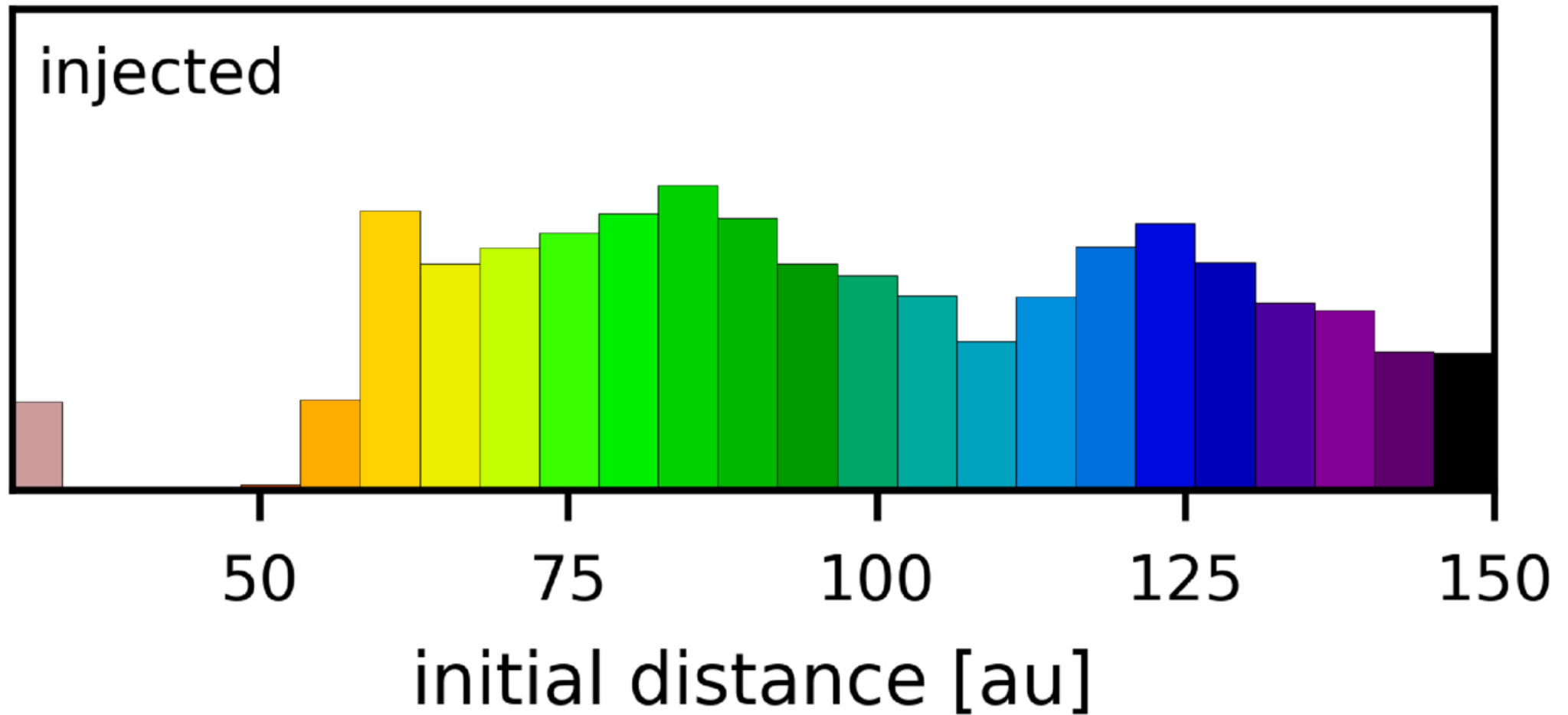
Figure D1. from Susanne Pfalzner et al 2025 Astrophys. J. Lett. 992 doi:10.3847/2041-8213/ae0e74 https://dx.doi.org/10.3847/2041-8213/ae0e74 © 2025. The Author(s). Published by the American Astronomical Society.
