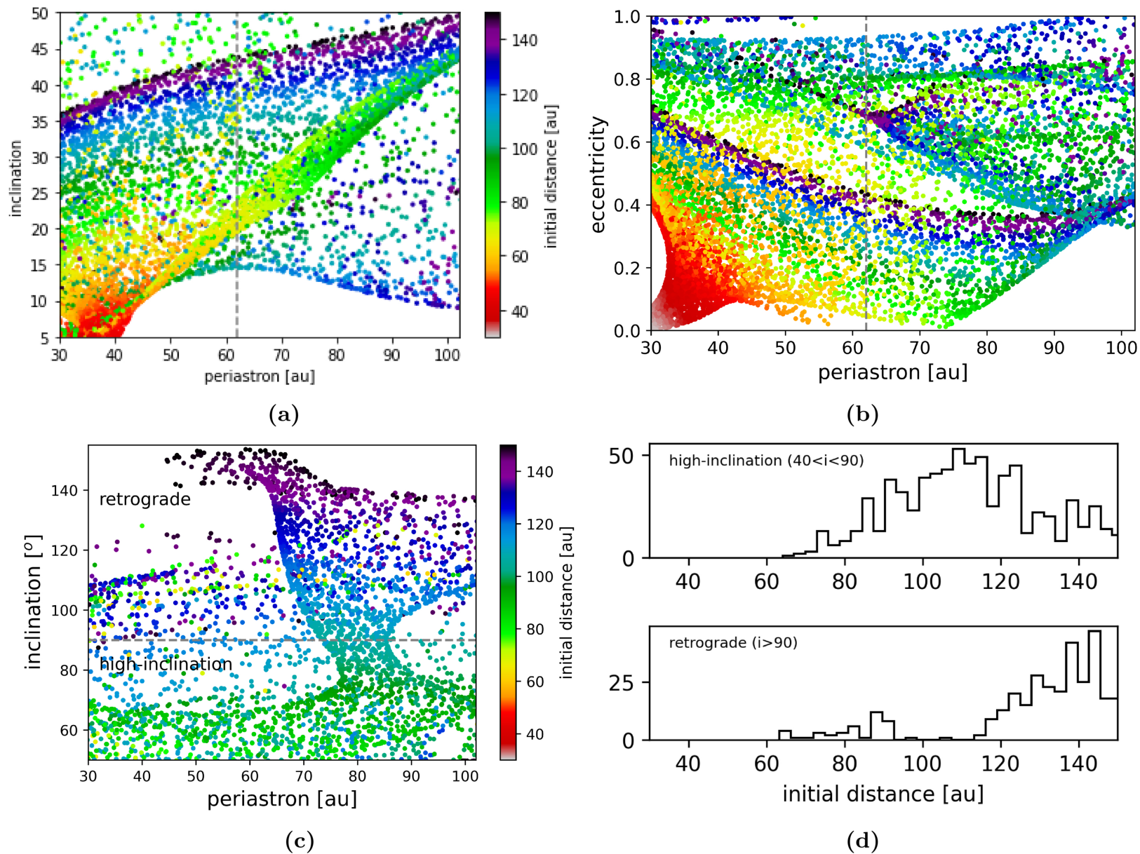
Figure 5. from Susanne Pfalzner et al 2025 Astrophys. J. Lett. 992 doi:10.3847/2041-8213/ae0e74 https://dx.doi.org/10.3847/2041-8213/ae0e74 © 2025. The Author(s). Published by the American Astronomical Society.
