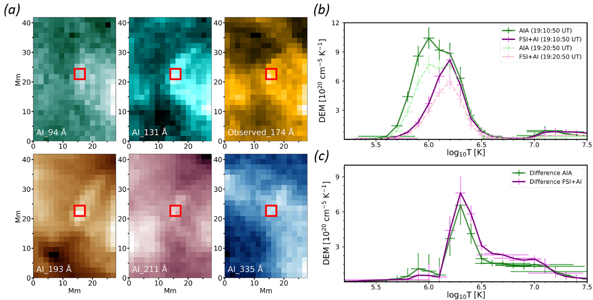
Figure 5. from Jeongwoo Lee et al 2025 Astrophys. J. Lett. 992 doi:10.3847/2041-8213/ae0df2 https://dx.doi.org/10.3847/2041-8213/ae0df2 © 2025. The Author(s). Published by the American Astronomical Society.
