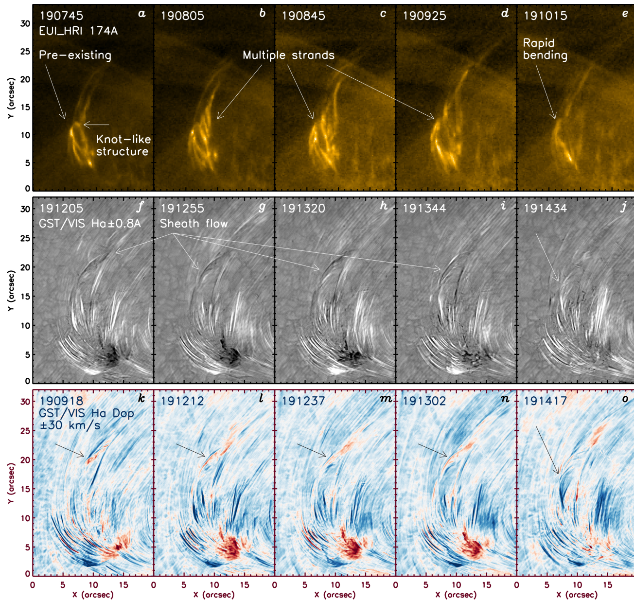
Figure 2. from Jeongwoo Lee et al 2025 Astrophys. J. Lett. 992 doi:10.3847/2041-8213/ae0df2 https://dx.doi.org/10.3847/2041-8213/ae0df2 © 2025. The Author(s). Published by the American Astronomical Society.
