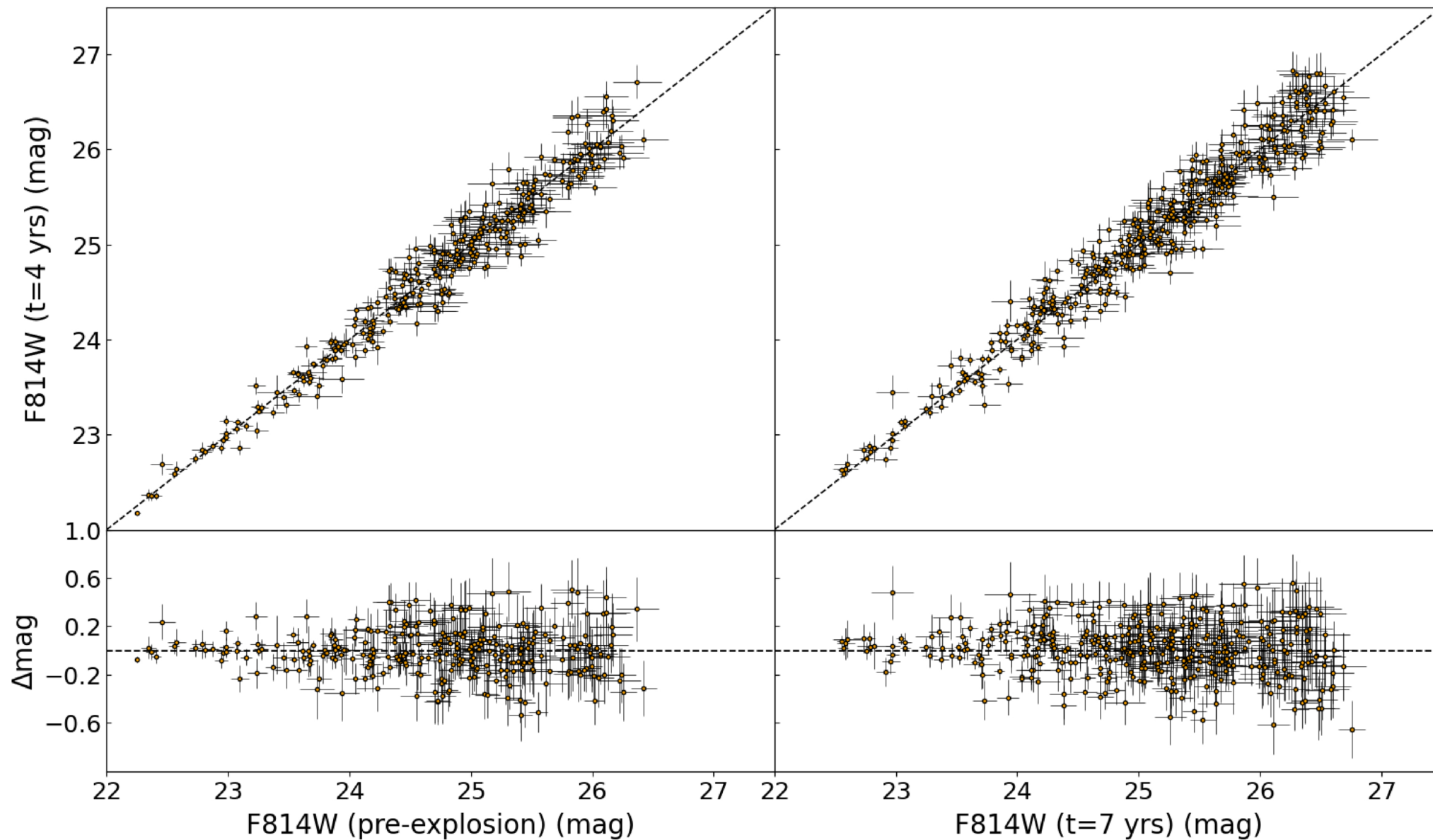
Figure 4. from Yi-Han Zhao et al 2025 Astrophys. J. Lett. 992 doi:10.3847/2041-8213/ae0d8f https://dx.doi.org/10.3847/2041-8213/ae0d8f © 2025. The Author(s). Published by the American Astronomical Society.
