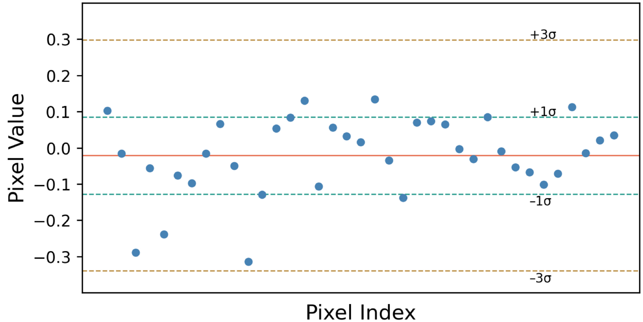
Figure 2. from Yi-Han Zhao et al 2025 Astrophys. J. Lett. 992 doi:10.3847/2041-8213/ae0d8f https://dx.doi.org/10.3847/2041-8213/ae0d8f © 2025. The Author(s). Published by the American Astronomical Society.
