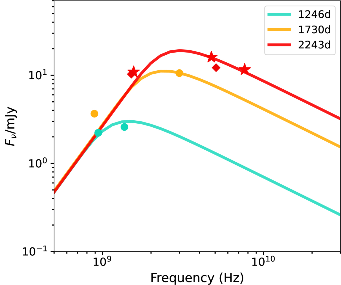
Figure 6. from Lei Yang et al 2025 Astrophys. J. Lett. 993 doi:10.3847/2041-8213/ae0caa https://dx.doi.org/10.3847/2041-8213/ae0caa © 2025. The Author(s). Published by the American Astronomical Society.
